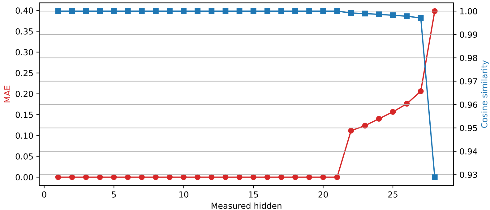
Llama-3.2-3B | Quantized layer 21 | float32 → int4
