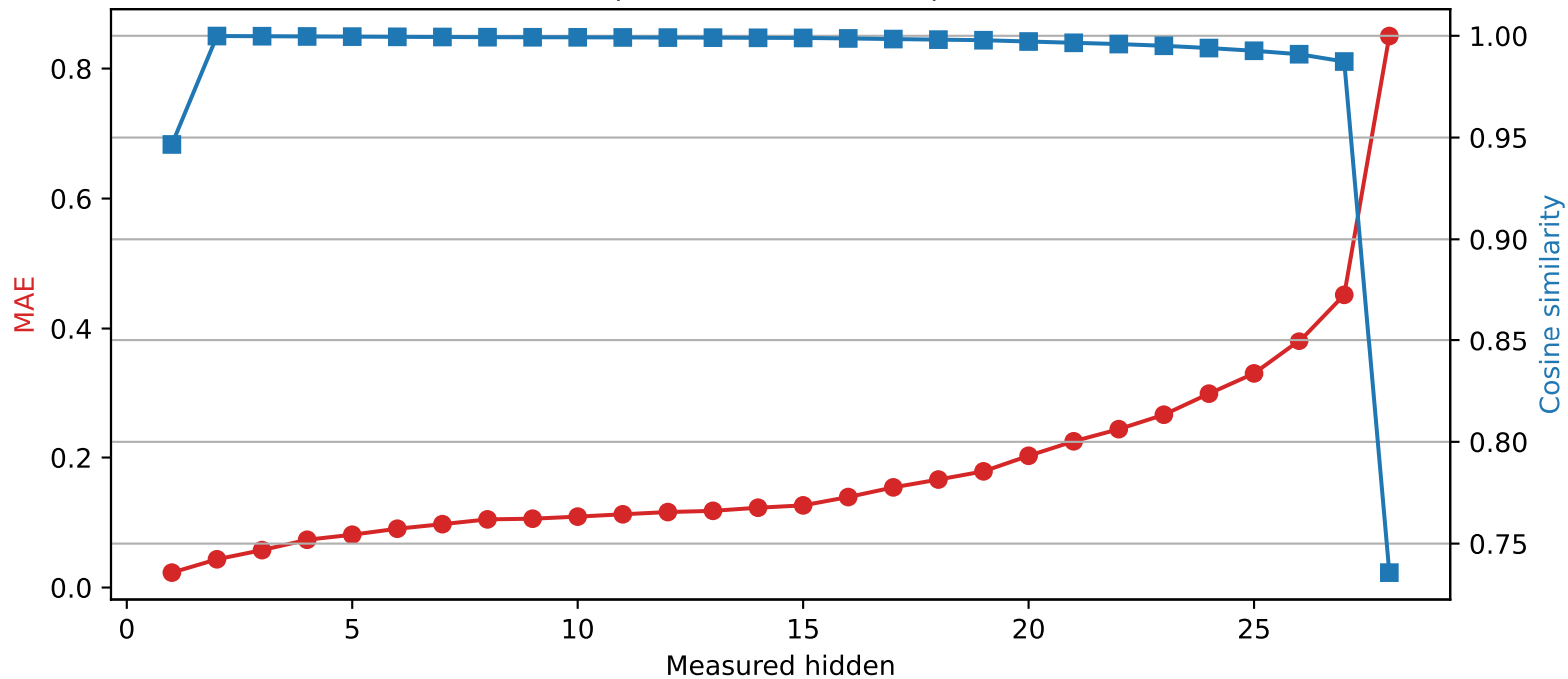
Llama-3.2-3B | Quantized layer 0 | float32 → int4
