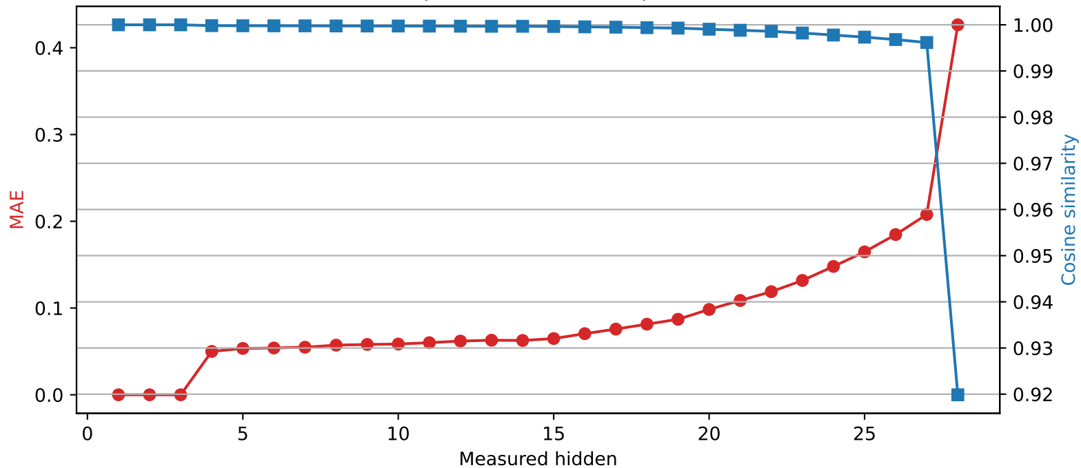
Llama-3.2-3B | Quantized layer 3 | float32 → int4
