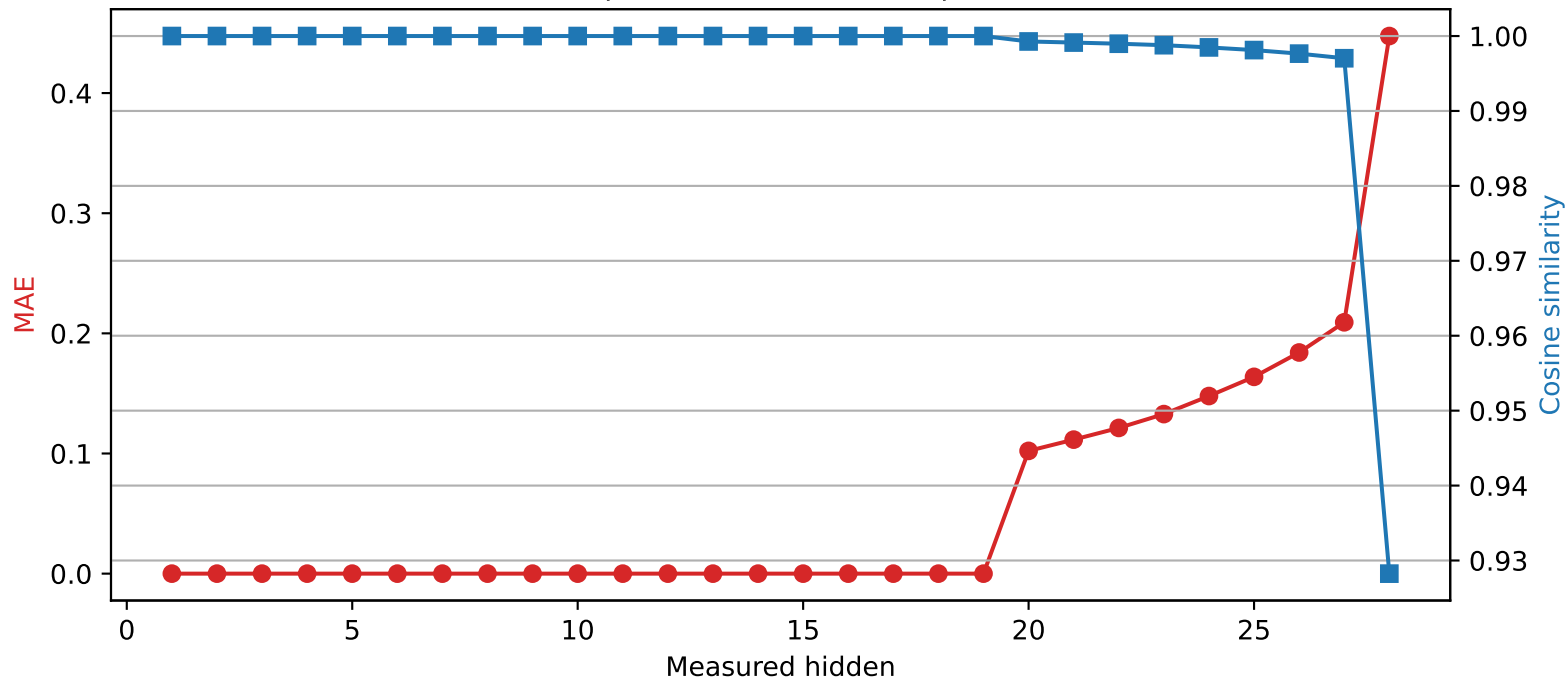
Llama-3.2-3B | Quantized layer 19 | float32 → int4
