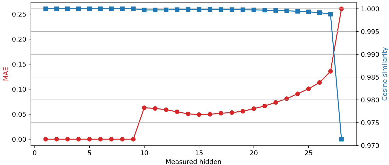
Llama-3.2-3B | Quantized layer 9 | float32 \rightarrow int4
