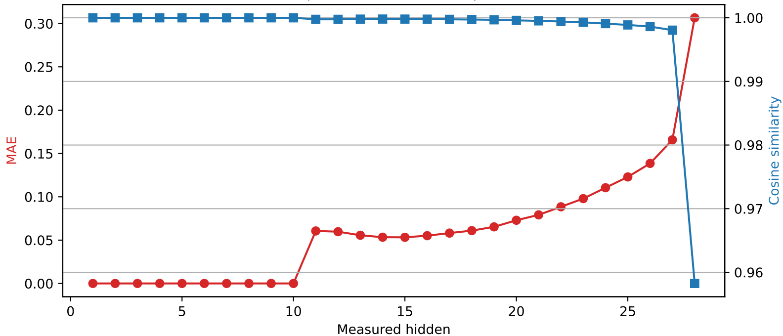
Llama-3.2-3B | Quantized layer 10 | float32 \rightarrow int4
