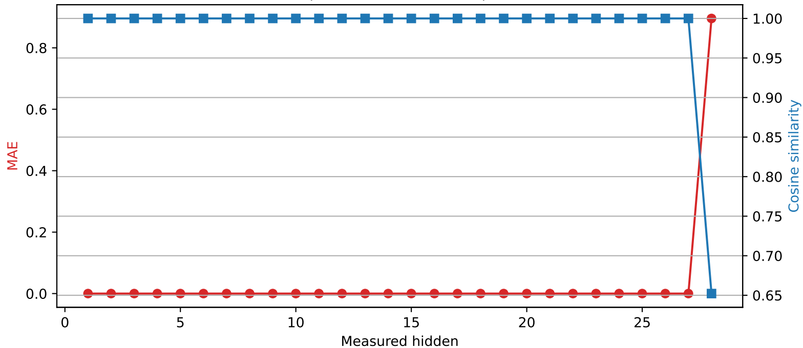
Llama-3.2-3B | Quantized layer 27 | float32 \rightarrow int4
