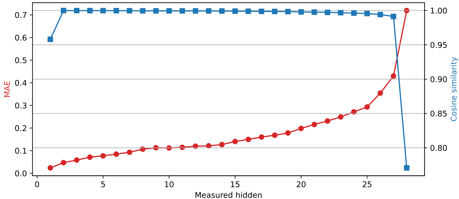
Llama-3.2-3B | Quantized layer 0 | float32 \rightarrow int4
