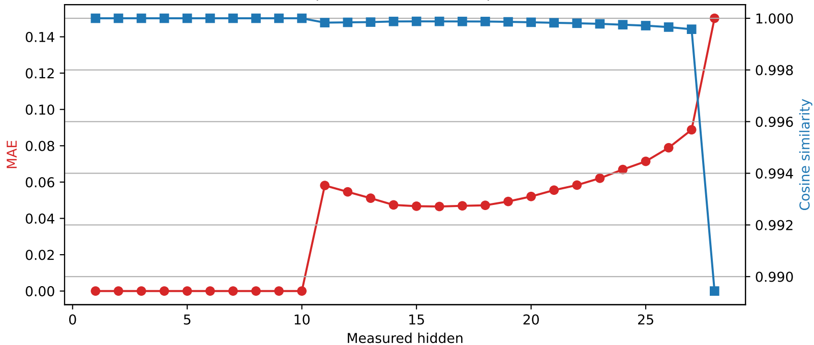
Llama-3.2-3B | Quantized layer 10 | float32 → int4
