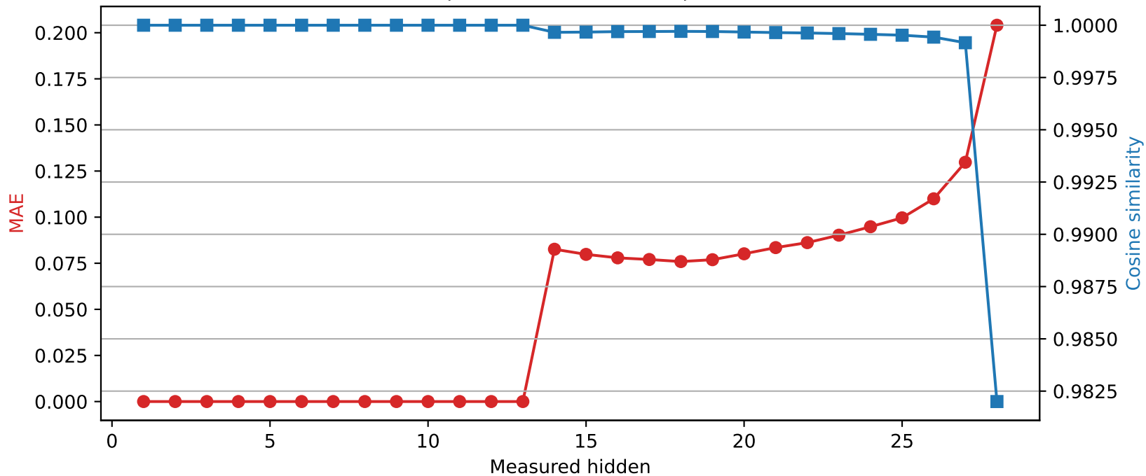
Llama-3.2-3B | Quantized layer 13 | float32 → int4
