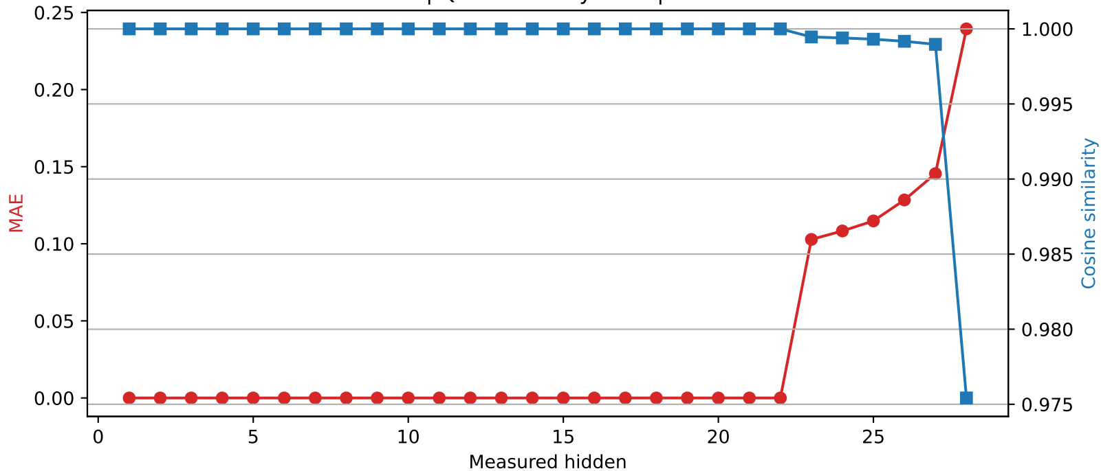
Llama-3.2-3B | Quantized layer 22 | float32 \rightarrow int4
