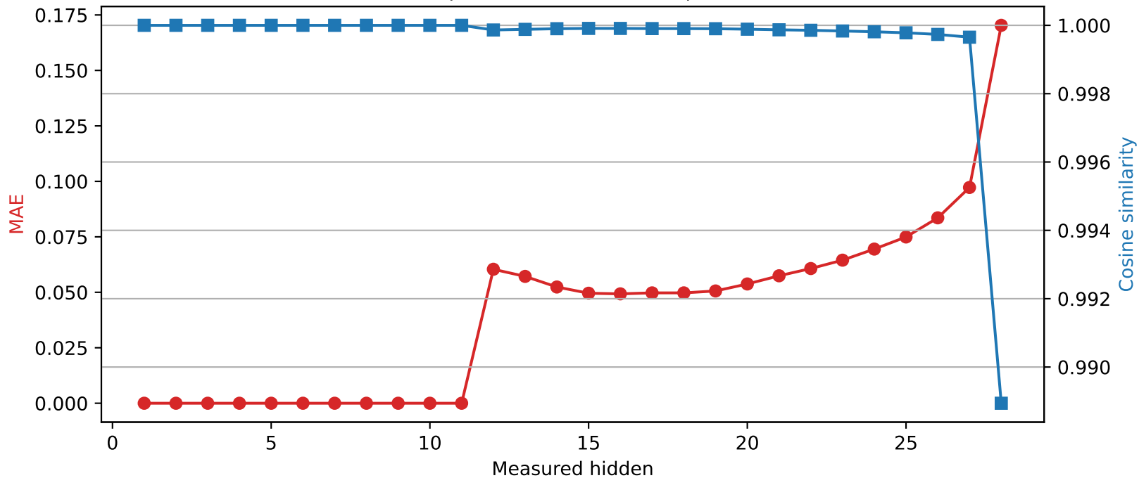
Llama-3.2-3B | Quantized layer 11 | float64 → int4
