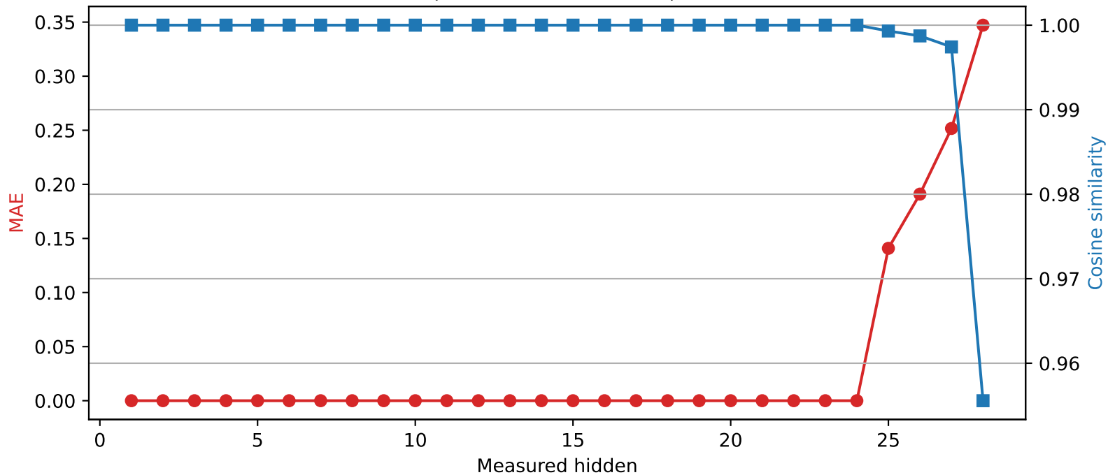
Llama-3.2-3B | Quantized layer 24 | float64 \rightarrow int4
