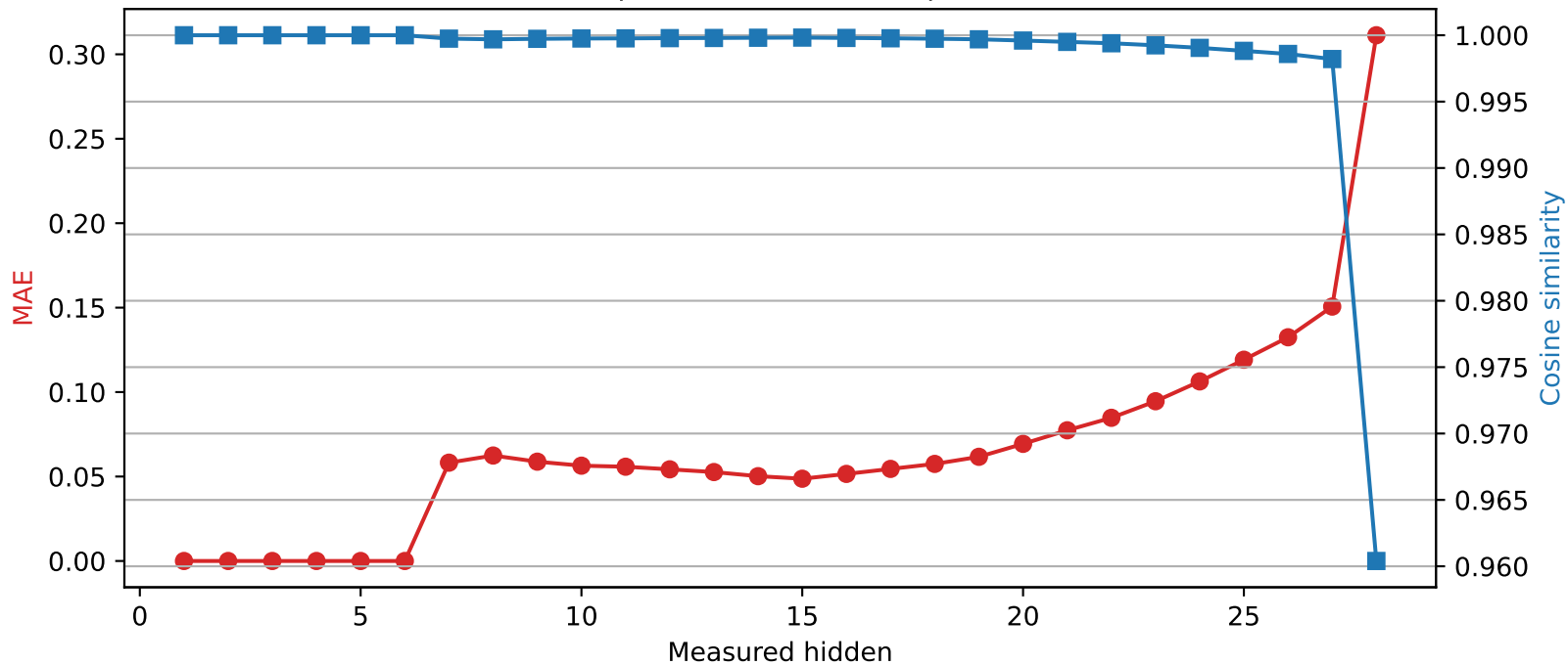
Llama-3.2-3B | Quantized layer 6 | float64 → int4
