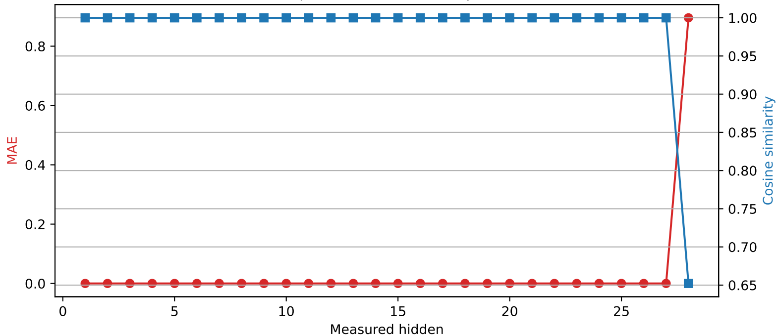
Llama-3.2-3B | Quantized layer 27 | float64 → int4
