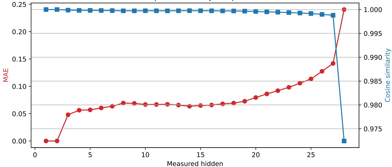
Llama-3.2-3B | Quantized layer 2 | float64 → int4
