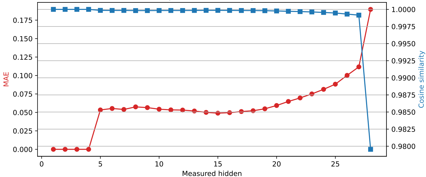
Llama-3.2-3B | Quantized layer 4 | float64 → int4
