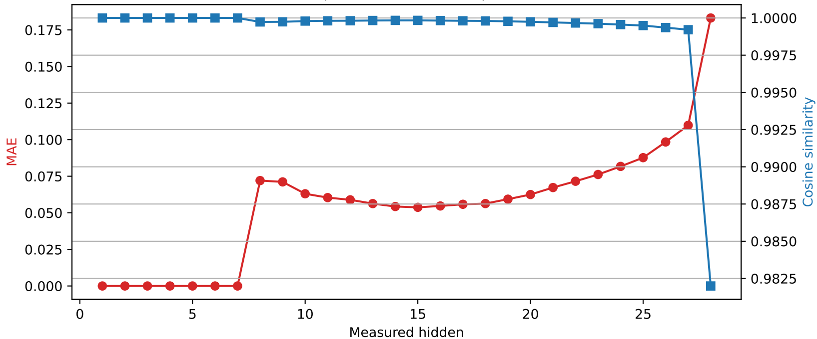
Llama-3.2-3B | Quantized layer 7 | float64 → int4
