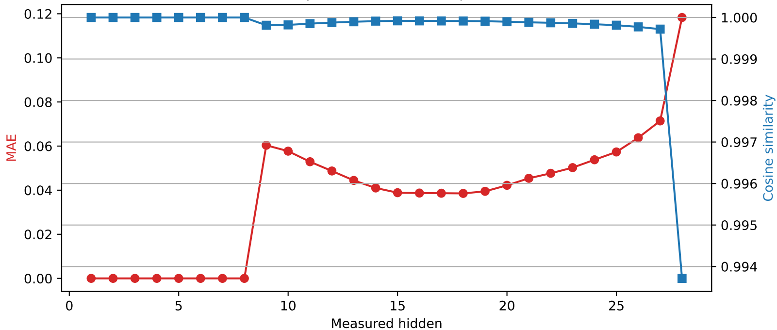
Llama-3.2-3B | Quantized layer 8 | float64 → int4
