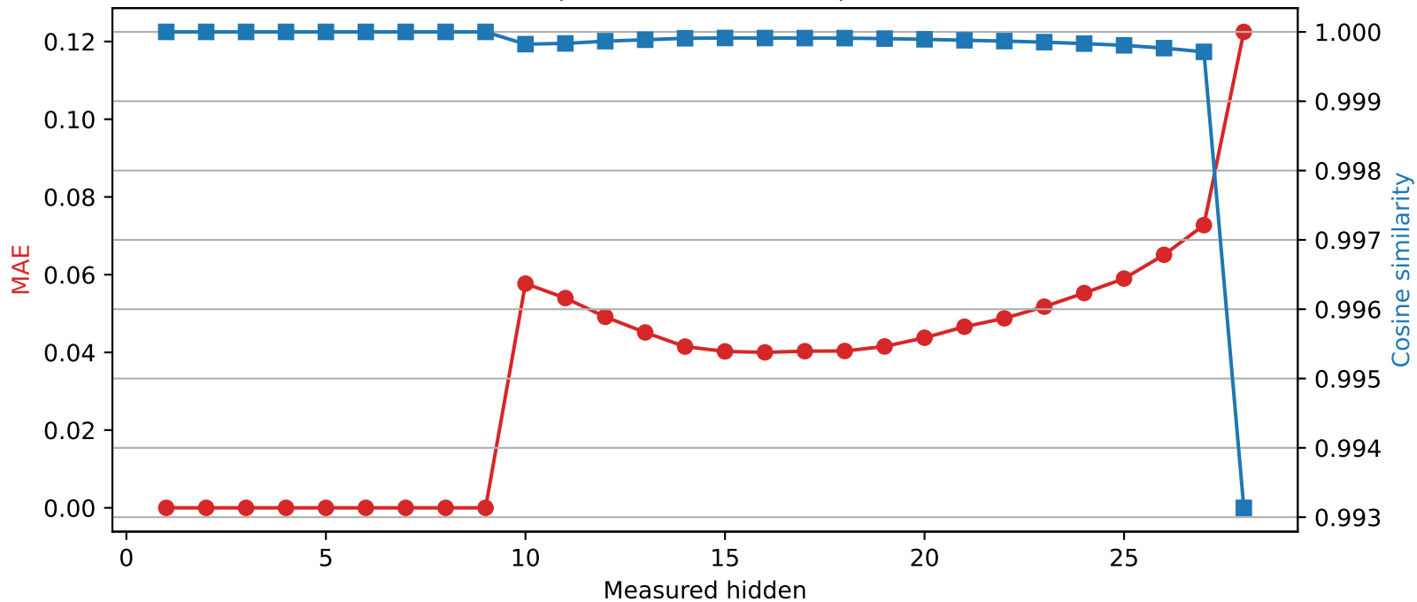
Llama-3.2-3B | Quantized layer 9 | float64 → int4
