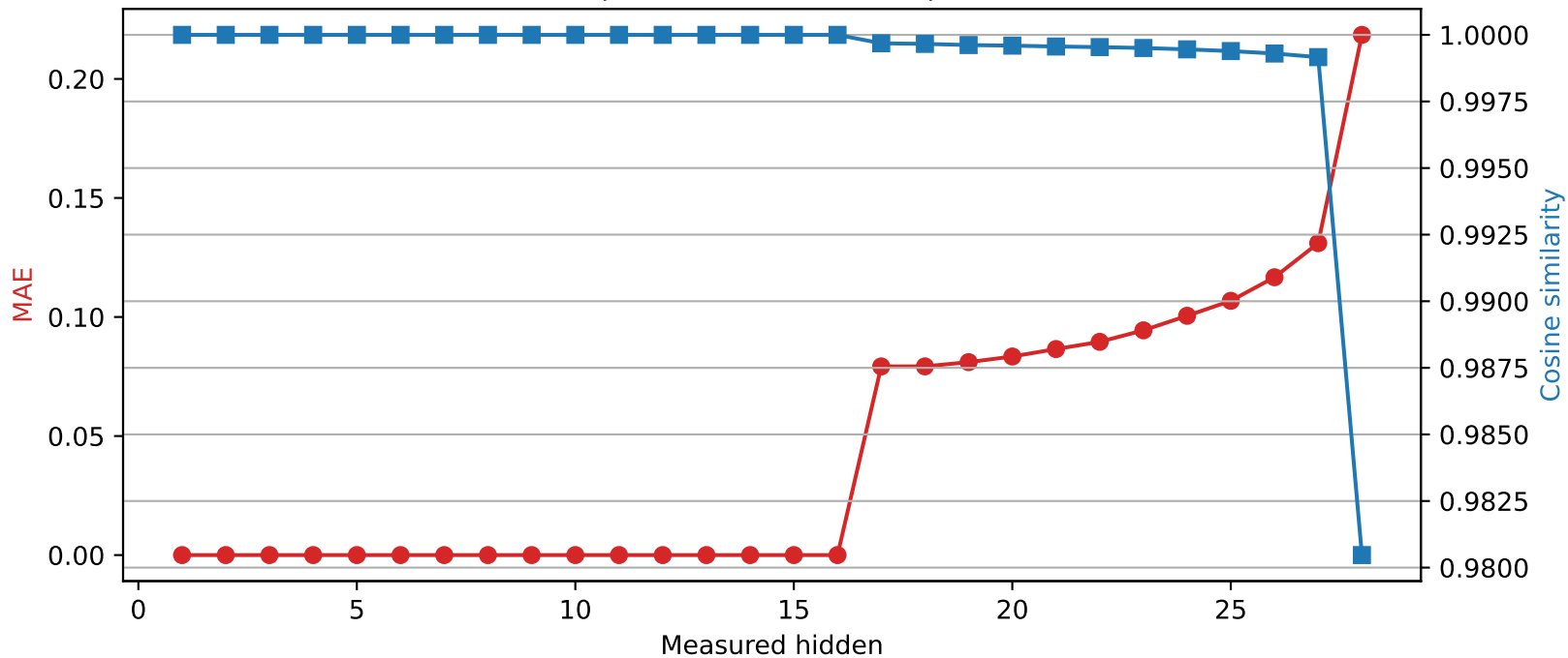
Llama-3.2-3B | Quantized layer 16 | float64 → int4
