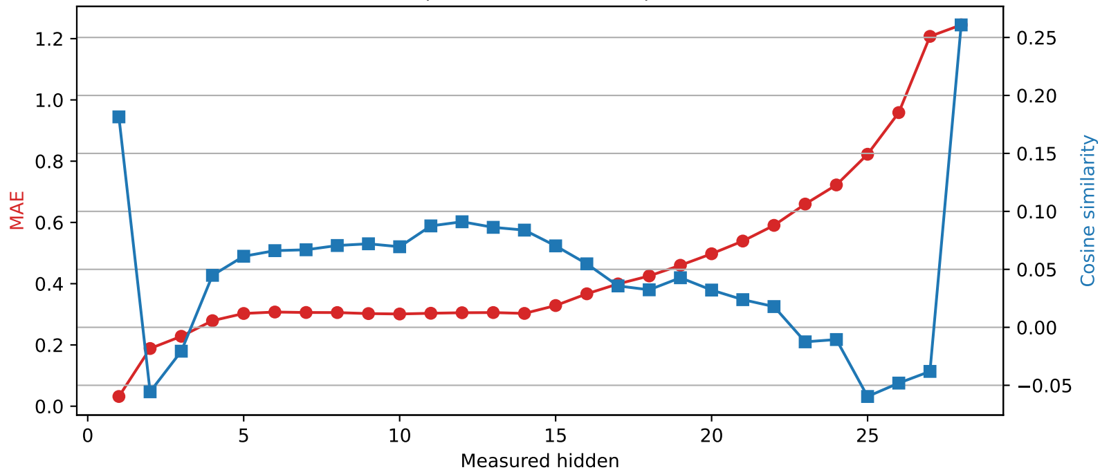
Llama-3.2-3B | Quantized layer 0 | float16 → int2
