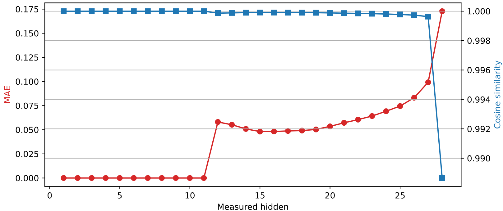
Llama-3.2-3B | Quantized layer 11 | float16 → int2
