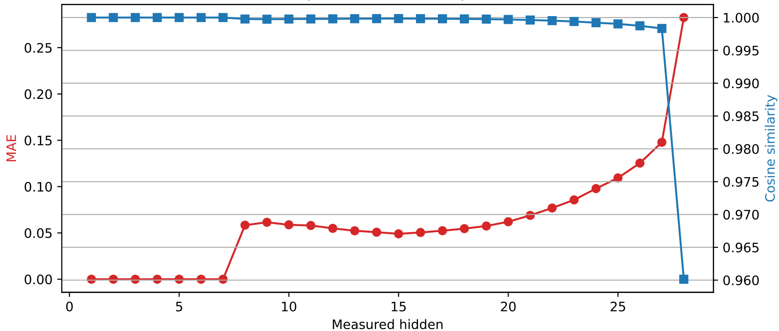
Llama-3.2-3B | Quantized layer 7 | float16 → int2
