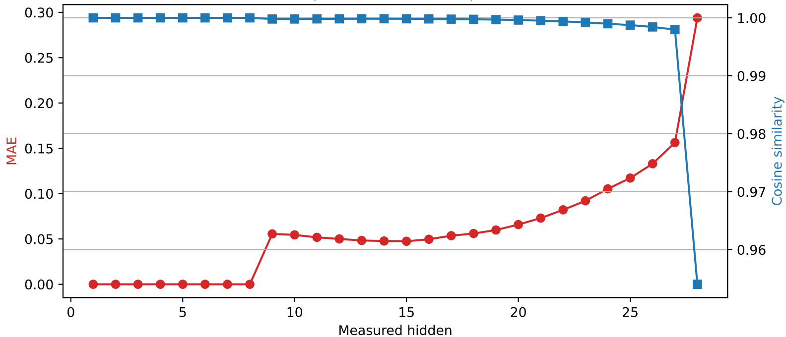
Llama-3.2-3B | Quantized layer 8 | float16 \rightarrow int2
