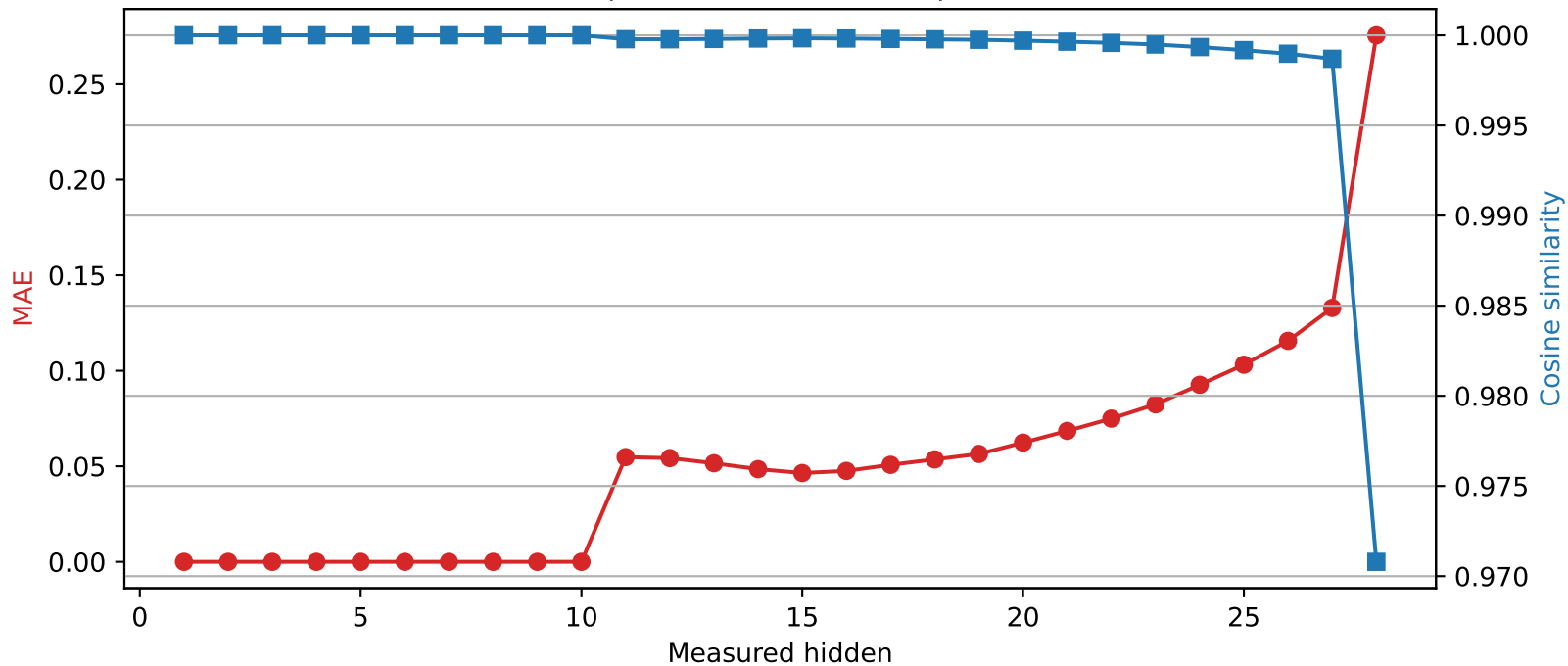
Llama-3.2-3B | Quantized layer 10 | float16 → int2
