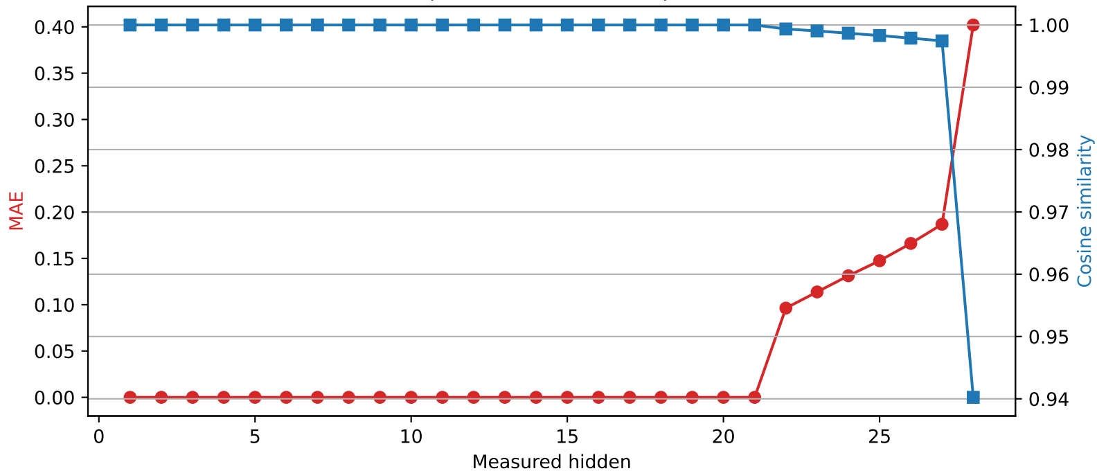
Llama-3.2-3B | Quantized layer 21 | float16 → int2
