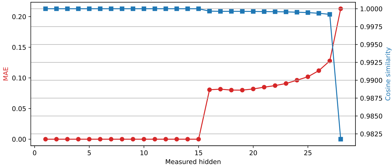
Llama-3.2-3B | Quantized layer 15 | float16 → int2
