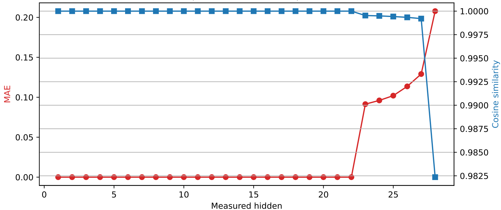
Llama-3.2-3B | Quantized layer 22 | float16 → int2
