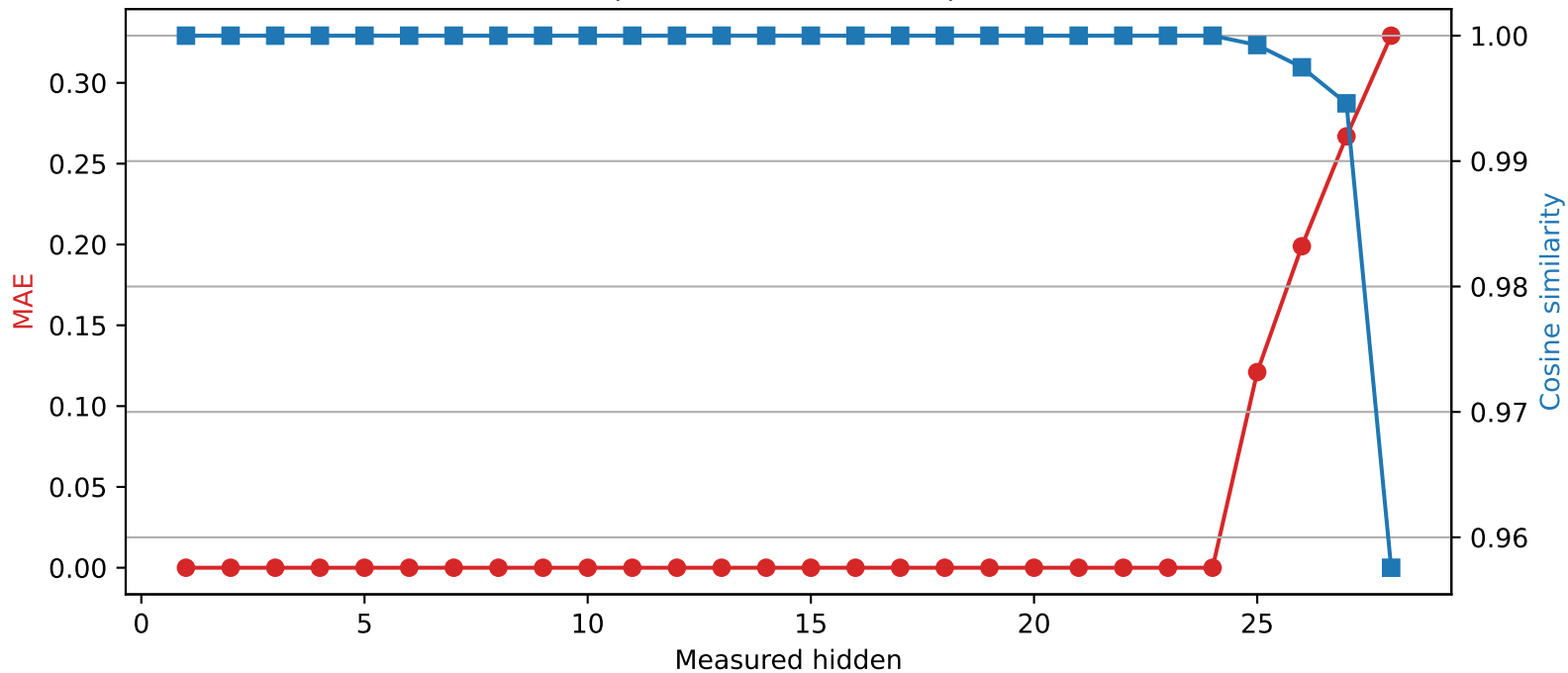
Llama-3.2-3B | Quantized layer 24 | float16 → int2
