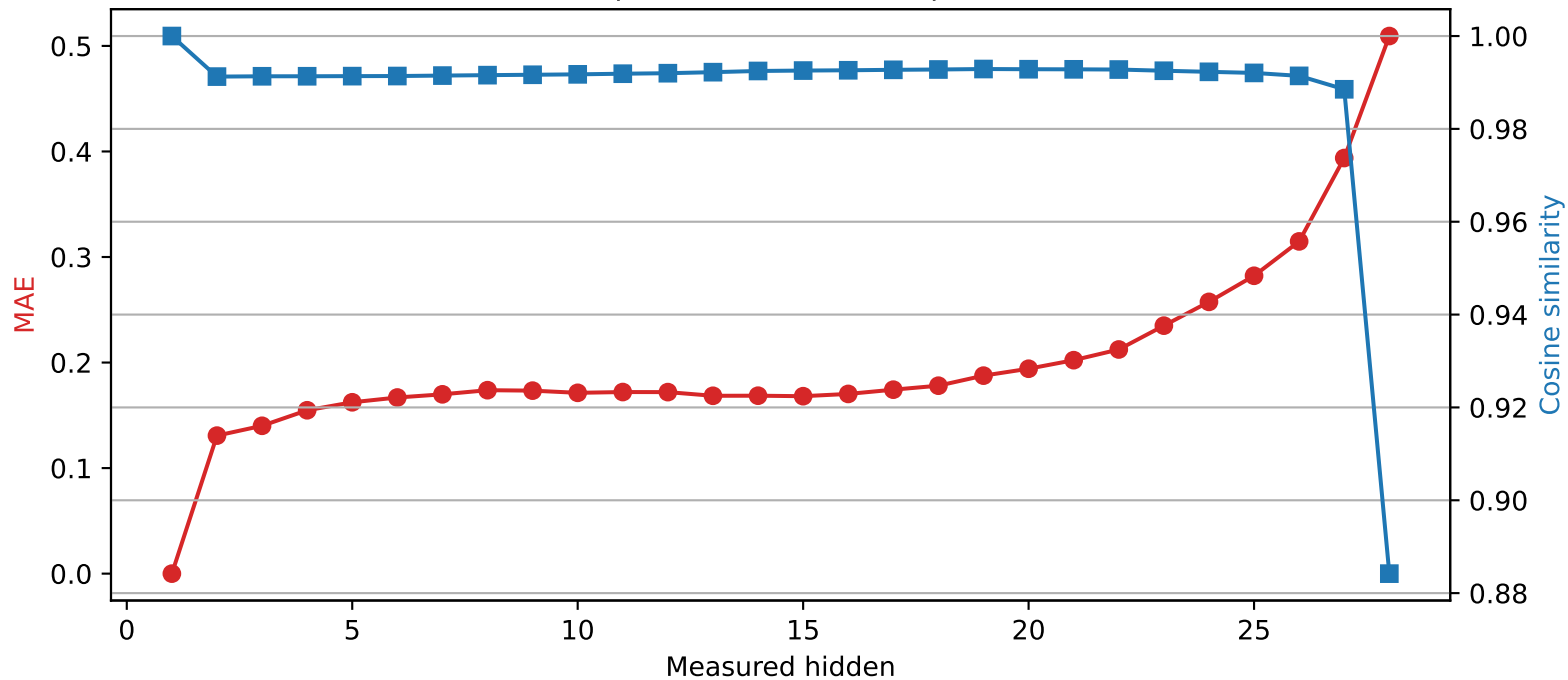
Llama-3.2-3B | Quantized layer 1 | float32 → int2
