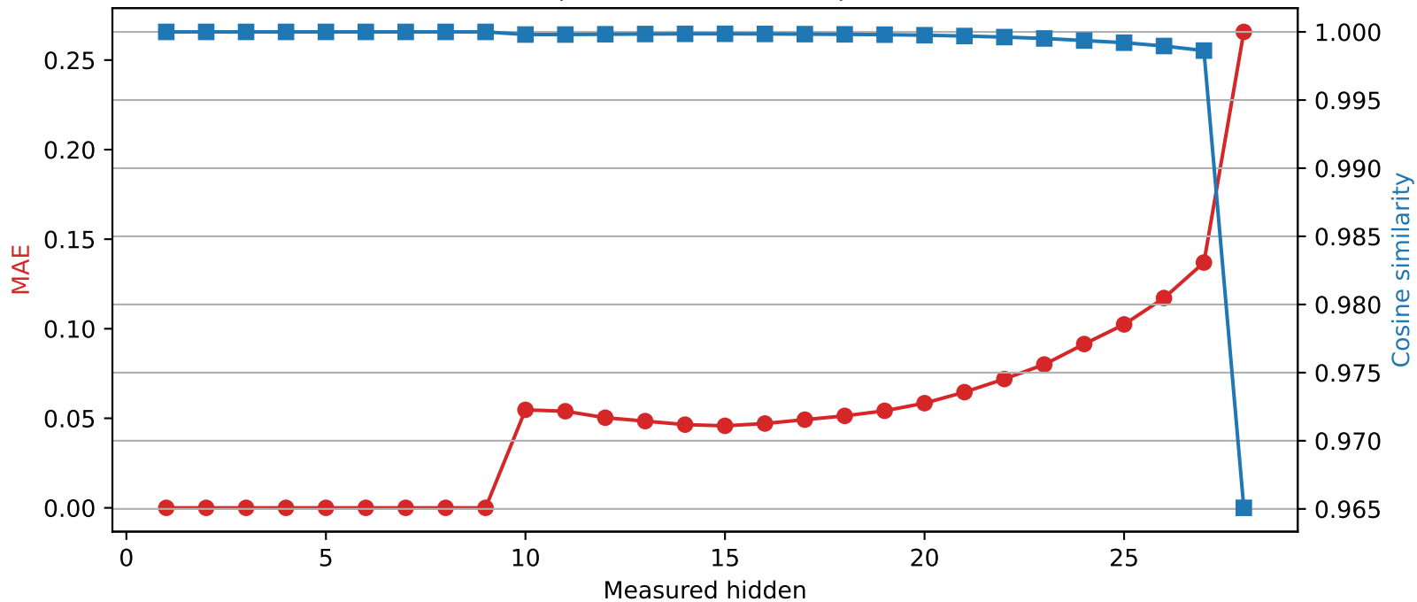
Llama-3.2-3B | Quantized layer 9 | float32 → int2
