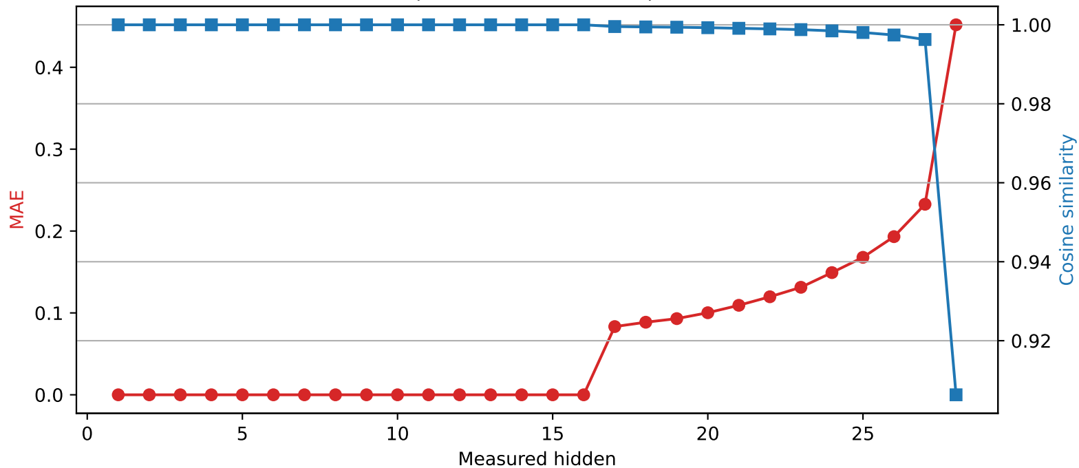
Llama-3.2-3B | Quantized layer 16 | float32 → int2
