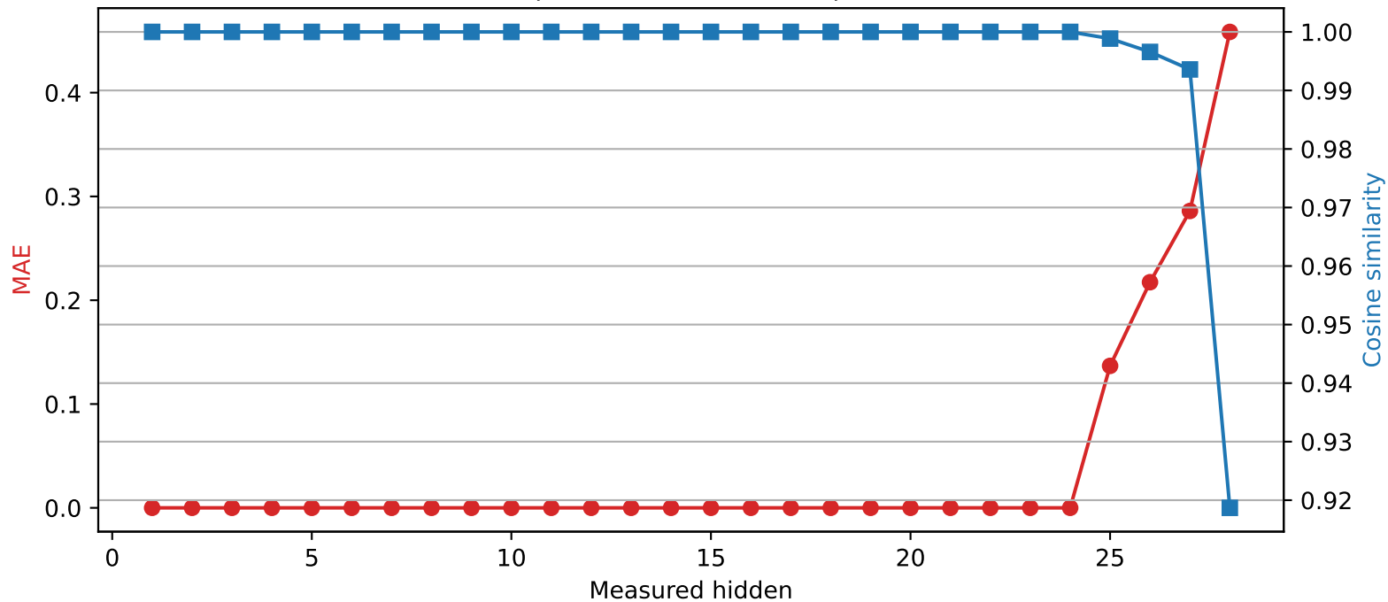
Llama-3.2-3B | Quantized layer 24 | float32 → int2
