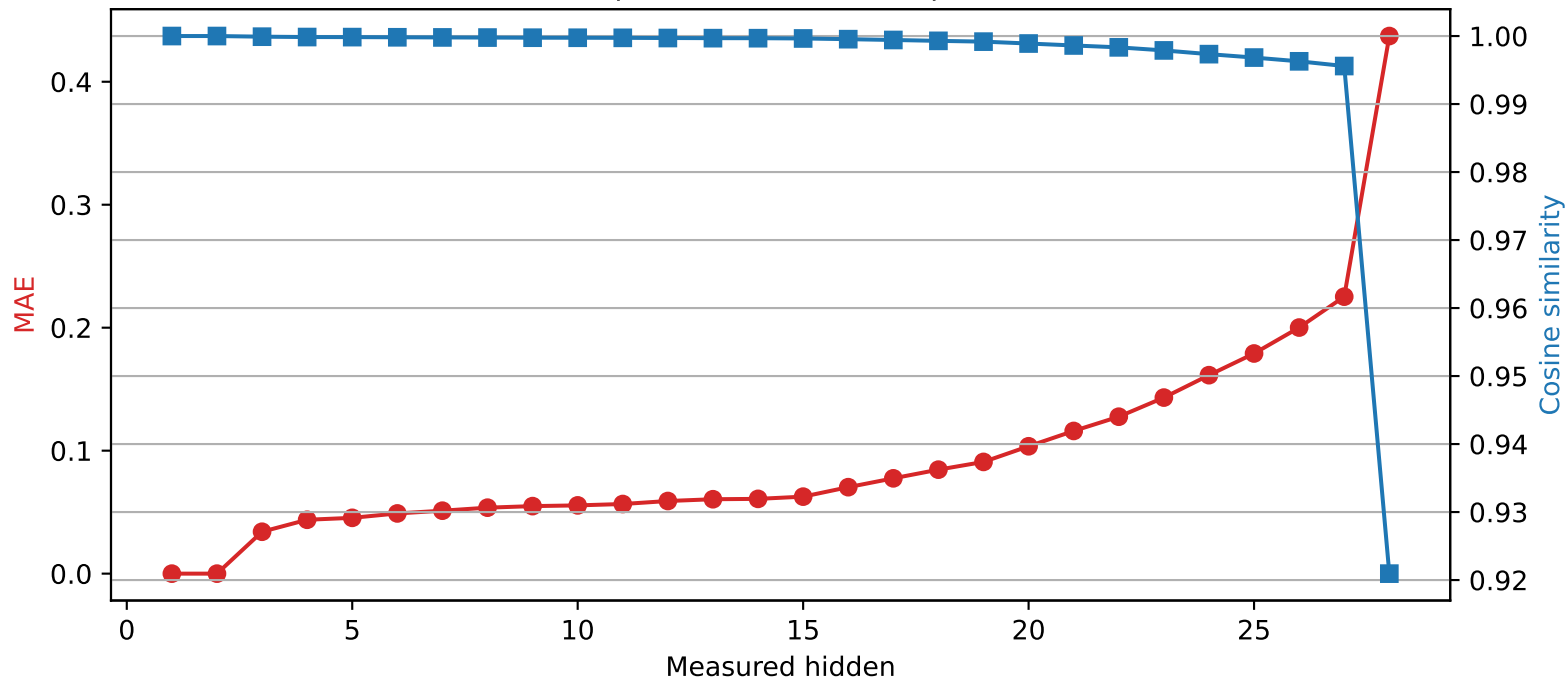
Llama-3.2-3B | Quantized layer 2 | float32 → int2
