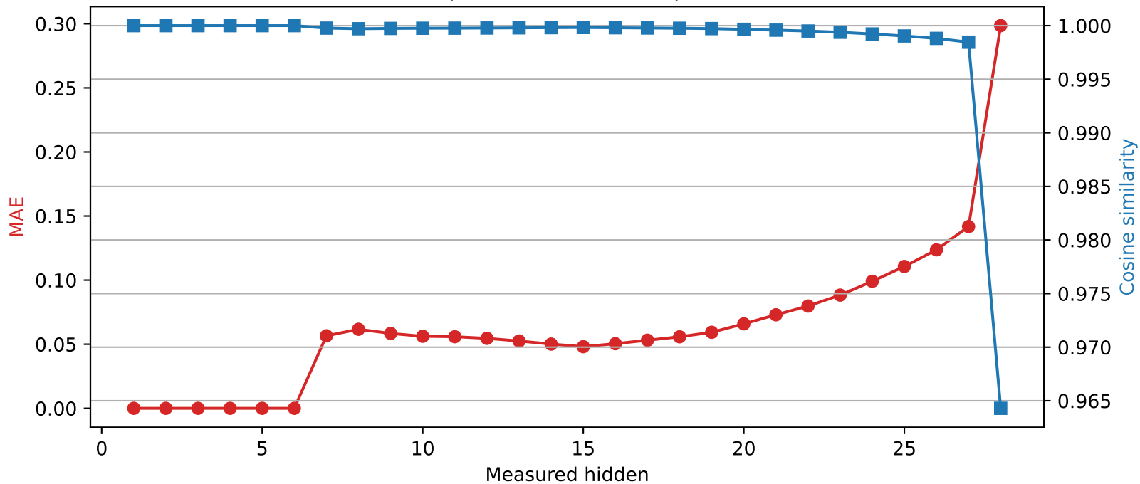
Llama-3.2-3B | Quantized layer 6 | float32 → int2
