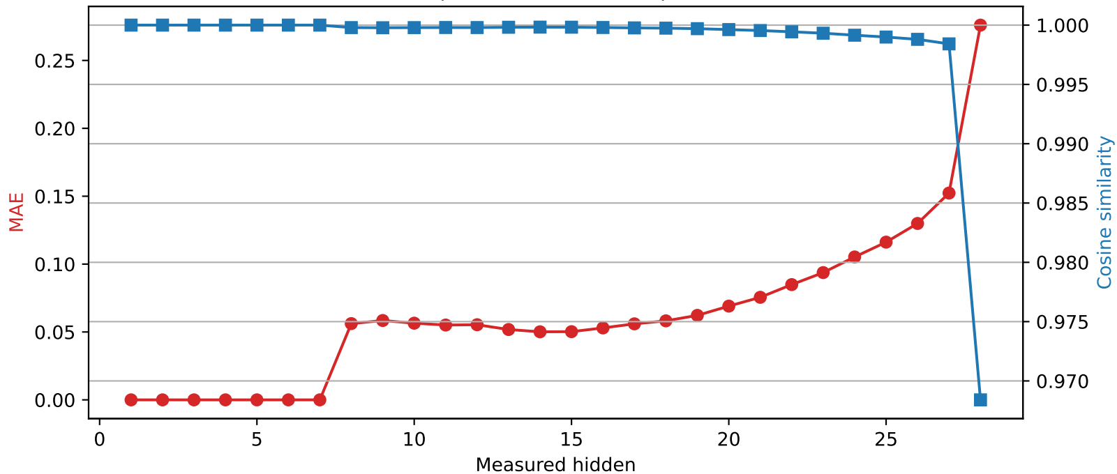
Llama-3.2-3B | Quantized layer 7 | float32 → int2
