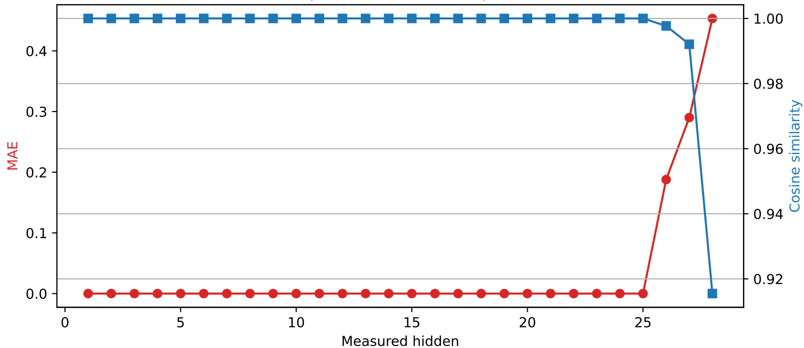
Llama-3.2-3B | Quantized layer 25 | float32 → int2
