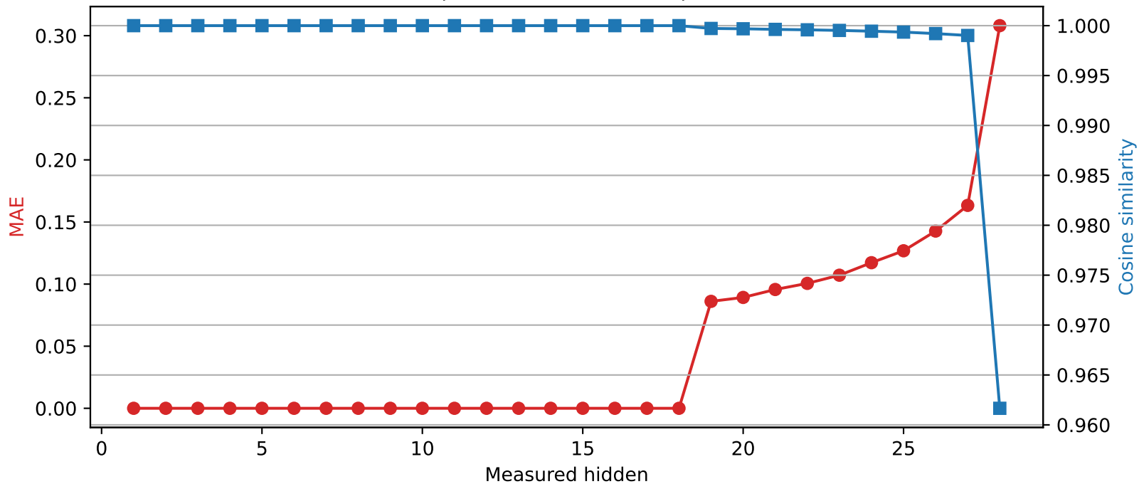
Llama-3.2-3B | Quantized layer 18 | float64 → int2
