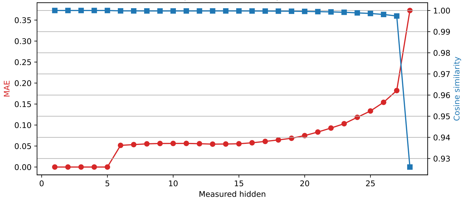
Llama-3.2-3B | Quantized layer 5 | float64 → int2
