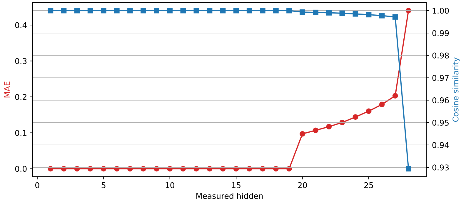
Llama-3.2-3B | Quantized layer 19 | float64 → int2
