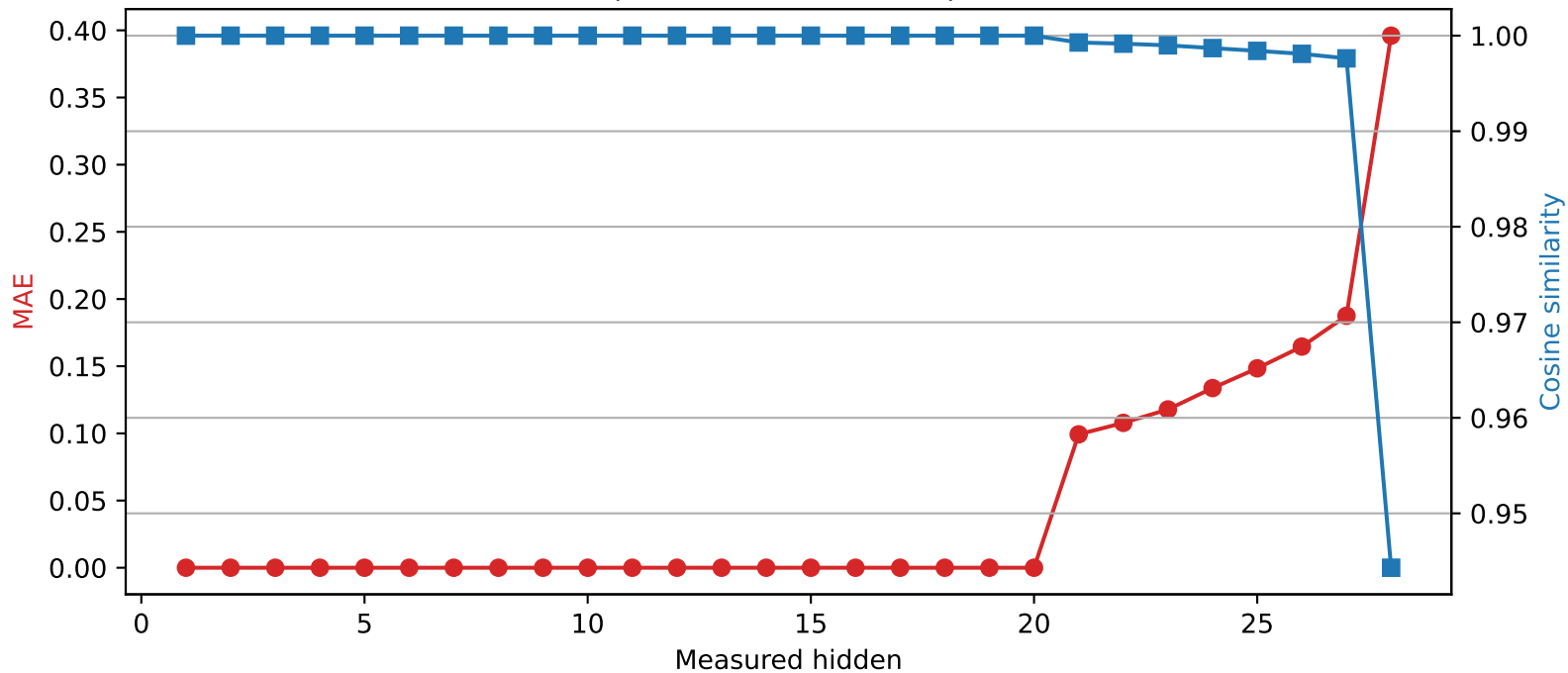
Llama-3.2-3B | Quantized layer 20 | float64 → int2
