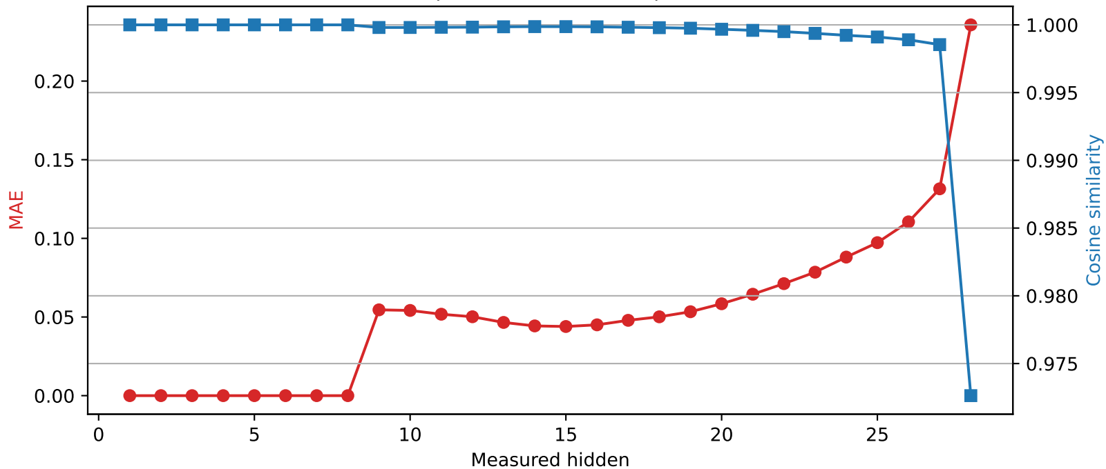
Llama-3.2-3B | Quantized layer 8 | float64 → int2
