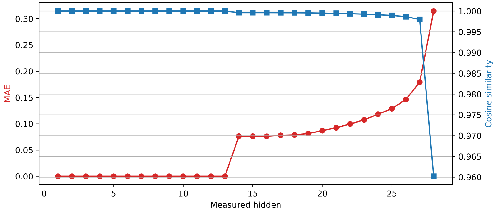
Llama-3.2-3B | Quantized layer 13 | float64 → int2
