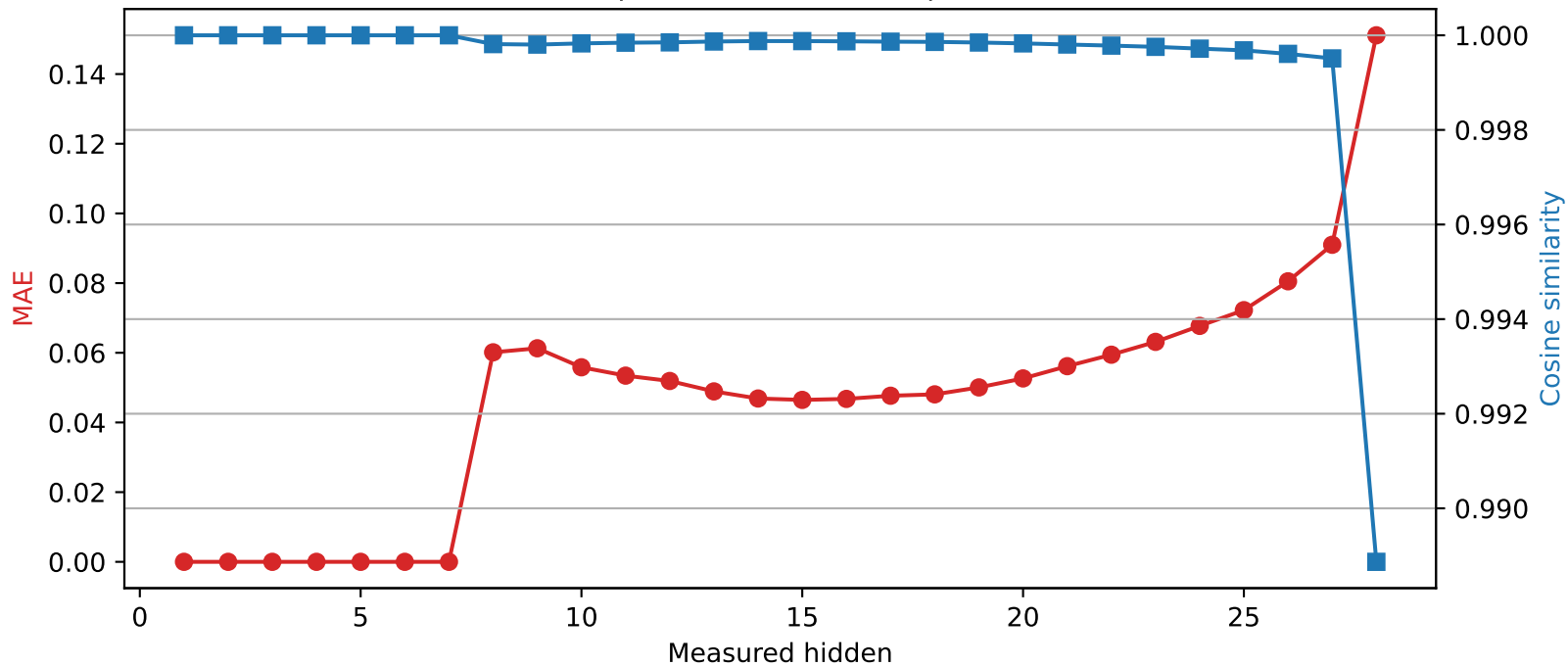
Llama-3.2-3B | Quantized layer 7 | float64 → int2
