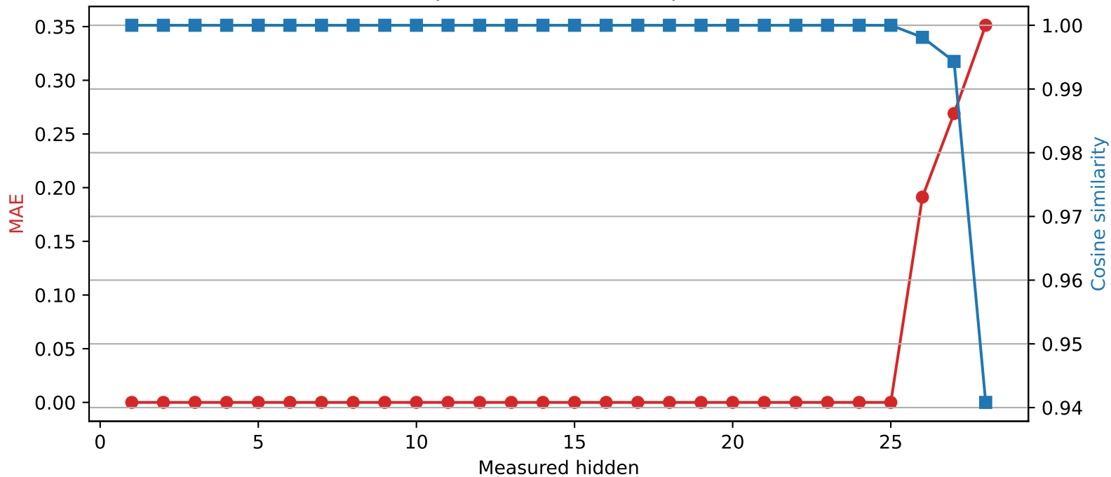
Llama-3.2-3B | Quantized layer 25 | float64 → int2
