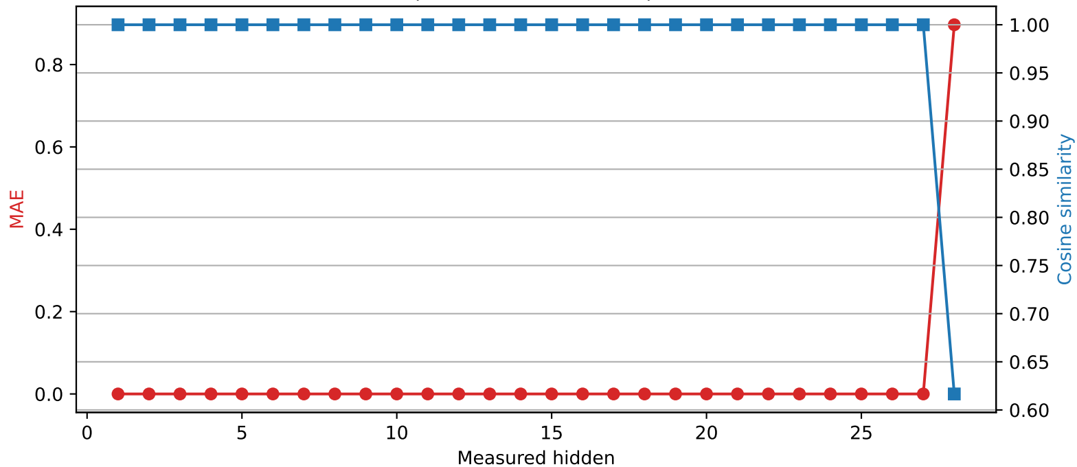
Llama-3.2-3B | Quantized layer 27 | float64 \rightarrow int2
