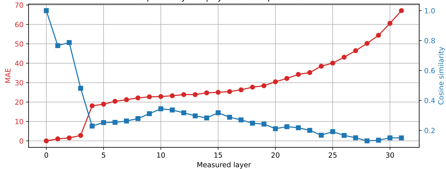
SmolLM2-360M | Prompt 0 Spared layer 1 | Hybrid vs unquantized
