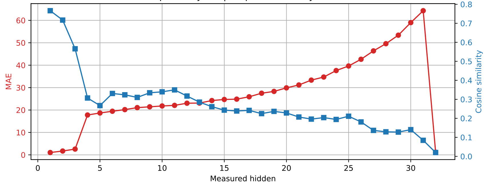
SmolLM2-360M | Prompt 0 Spared layer 5 | Unquantized vs hybrid
