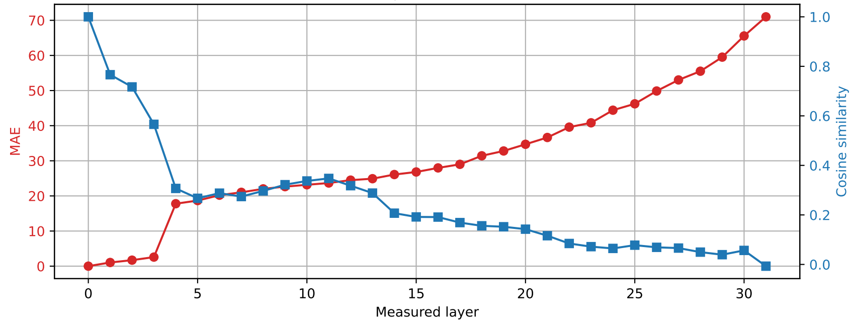
SmolLM2-360M | Prompt 0 Spared layer 8 | Hybrid vs unquantized
